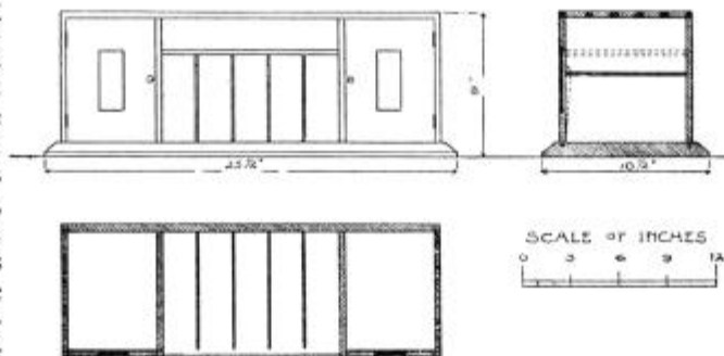
WORKING DRAWING OF PORTABLE CABINET.
