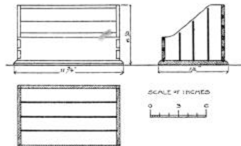
WORKING DRAWING OF LETTER FILE
