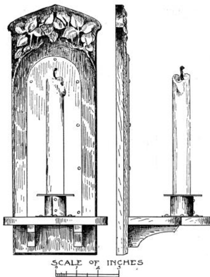
SCONCE NUMBER TWO
