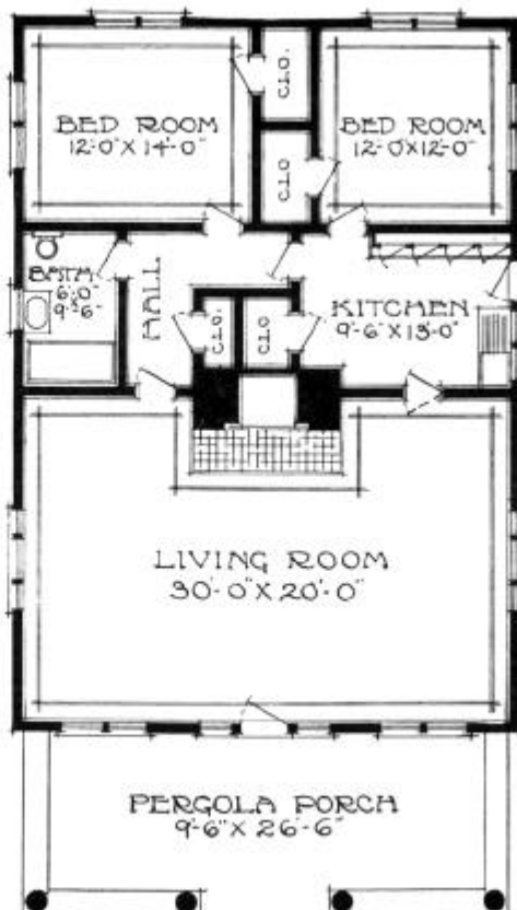
NO. 124: CRAFTSMAN CONCRETE BUNGALOW WITH PERGOLA PORCH
