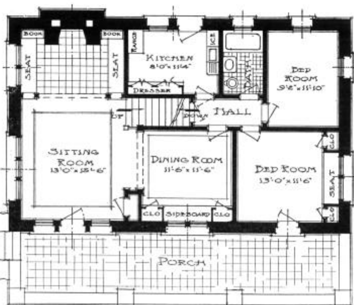
FLOOR PLAN OF STONE AND SHINGLE COTTAGE: NO. 93.
