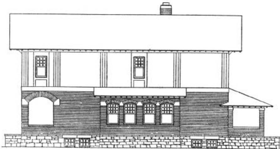
SIDE ELEVATION
