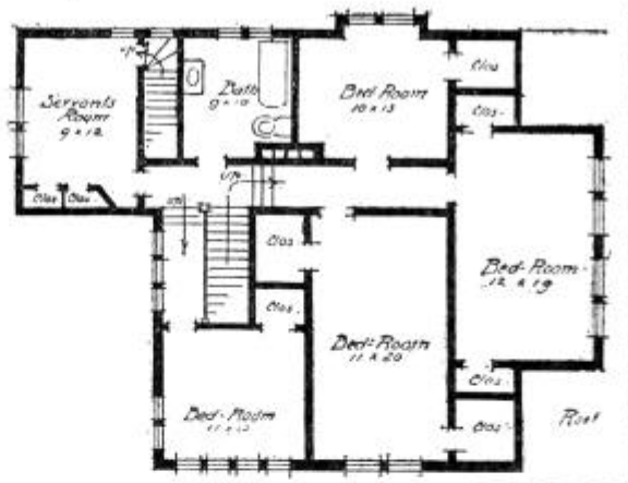
SECOND FLOOR PLAN OF MOUNTAIN COTTAGE.
