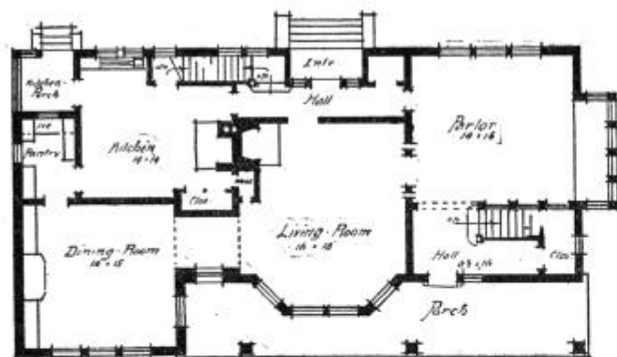
FIRST FLOOR PLAN FOR SUBURBAN COTTAGE.
