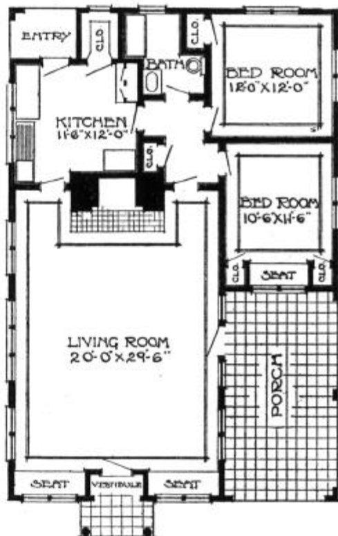
FLOOR PLAN OF BUNGALOW NO. 123.
