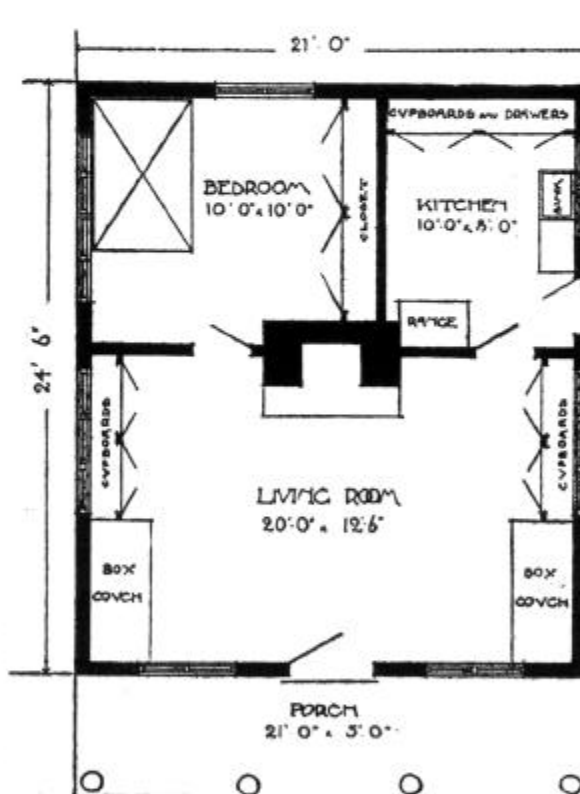
FLOOR PLAN FOR CRAFTSMAN BUNGALOW NUMBER TWO.
