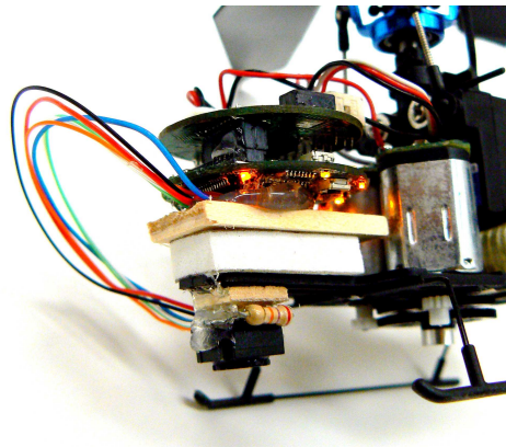
Figure 3.18: A downward pointing WiiMote camera is wired into a serial port on the GINA controller to enable the helicopter to hover over the IR beacon.
