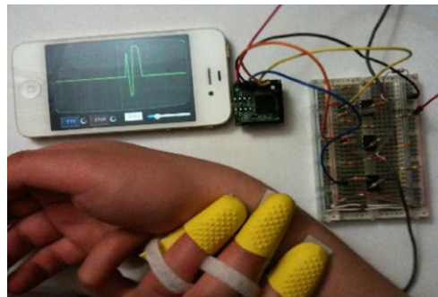
Figure 19 Dr.Chi prototype
