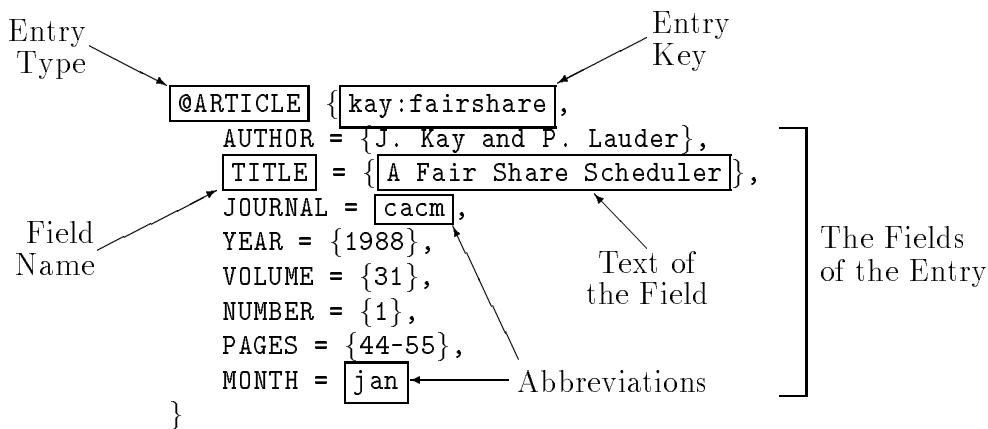
Figure 1: A sample entry from a BibTeX database file.
