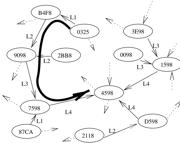
Figure 1: Tapestry routing example . Here we see the path taken by a message originating from node 0325 destined for node 4598 in a Tapestry network using hexadecimal digits of length 4 (65536 nodes in namespace).
