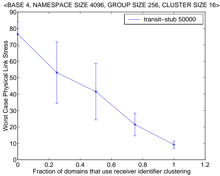
Figure 18: Worst case physical link stress vs. fraction of domains that use receiver ID clustering for the transit-stub model
