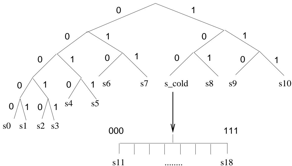
Figure 2-6: Modified entropy coding of the codevector indices. In this example, Huffman coding is used for codevectors in the hotlist plus the prefix of the rest of the codebook ( s_{cold} ). Fixed length codes then append s_{cold} . C_{hot} = \{s_0, \dots, s_{10}\} , C_{cold} = \{s_{11}, \dots, s_{18}\} .
