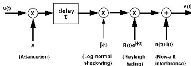
Figure 1: Fading channel model
