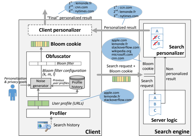
Fig. 2: Bloom cookies framework for web search.
