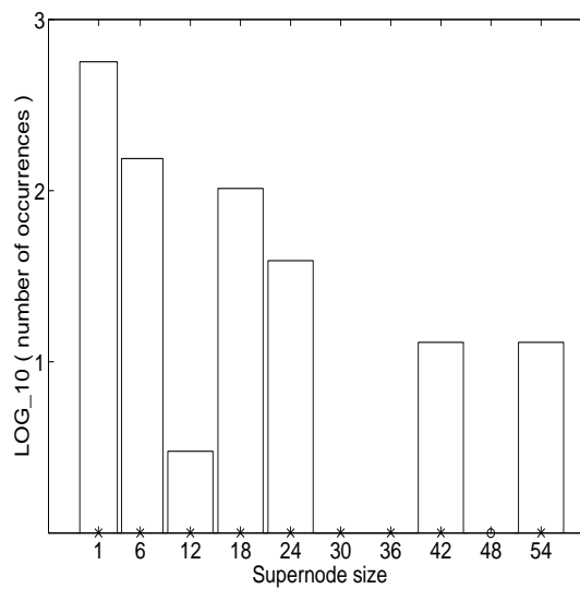
Figure 4.13: Distribution of supernode size for four matrices.
