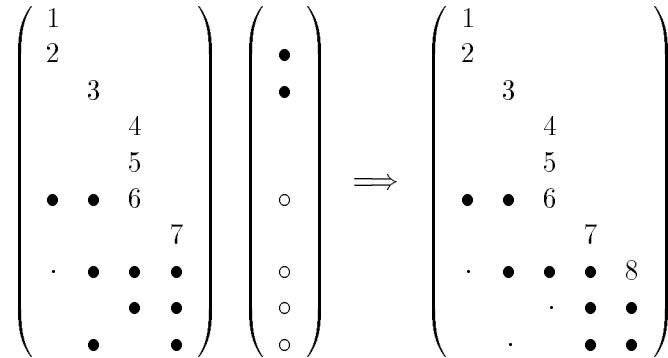
Figure 4.6: One step of symbolic factorization in the reduced structure.
